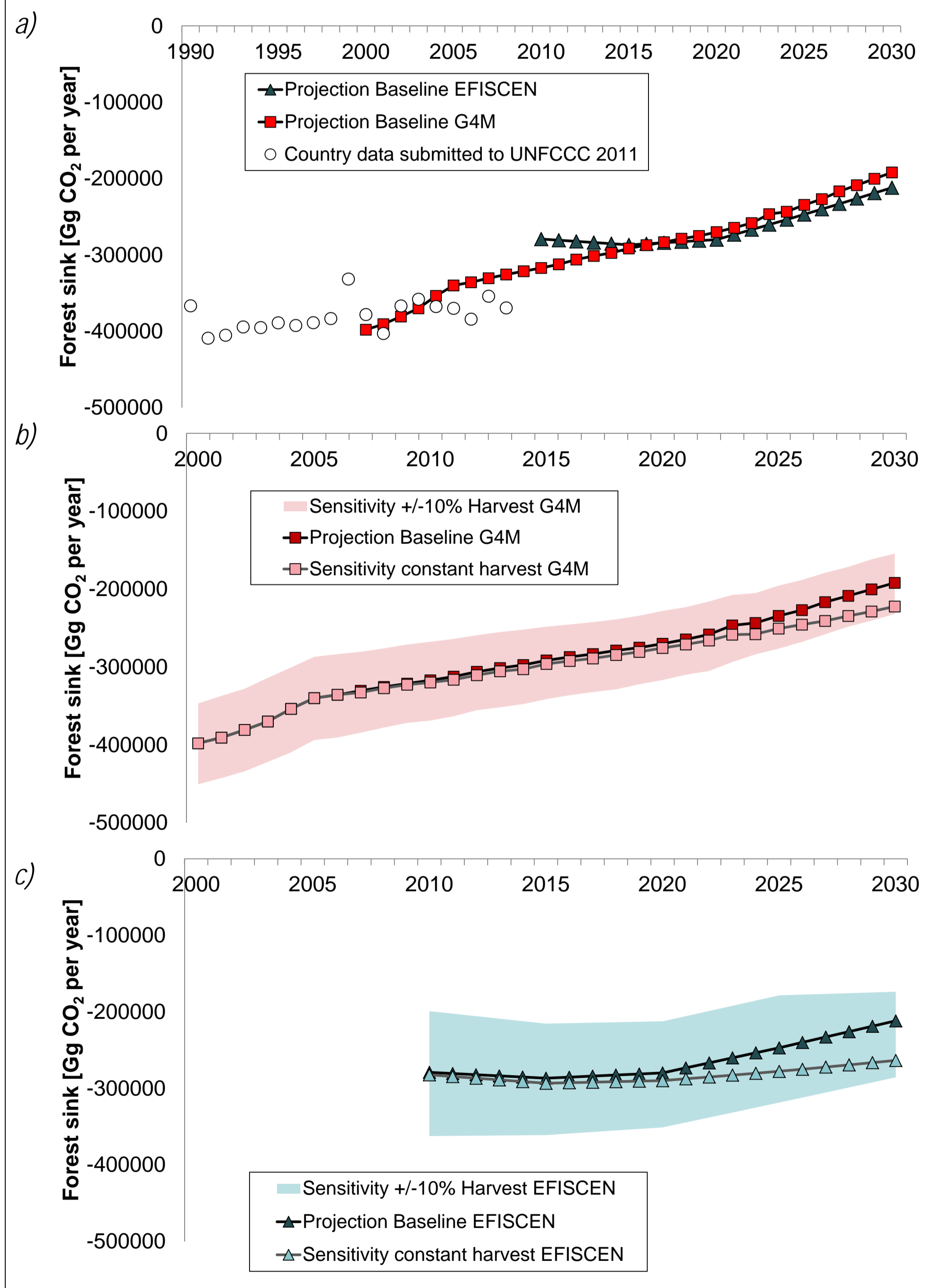
Fig. 1: Comparison of the forest management biomass sink from the model baselines and data submitted by countries to UNFCCC in May 2011 (a) and sensitivity runs for G4M (b) and EFISCEN (c) for EU member states (excl. Cyprus, Malta and Greece).
